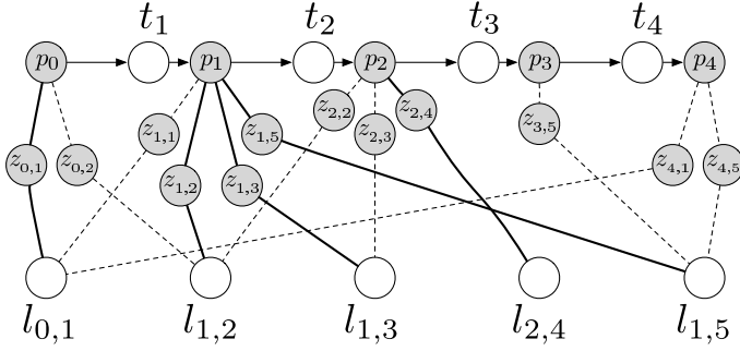
Figure 2. Graphical example for the sequence of 12 observations, \{z_{0,1}, z_{1,1}, z_{4,1}\}, \{z_{0,2}, z_{1,2}, z_{2,2}\}, \{z_{1,3}, z_{2,3}\}, \{z_{2,4}\}, \{z_{1,5}, z_{3,5}, z_{4,5}\} . There are five poses, p_0, \dots, p_4 , four edge estimates t_1, \dots, t_4 , and five landmarks l_{0,1}, l_{1,2}, l_{1,3}, l_{2,4} and l_{1,5} . This example has the Jacobian H = \frac{\partial h}{\partial x} that is depicted in Figure 3. Bold lines from poses indicate which frames are base-frames.
